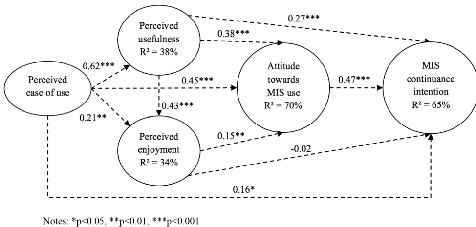
Figure 3: Female subgroup model
