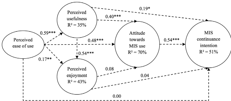
Figure 4: Male subgroup model
