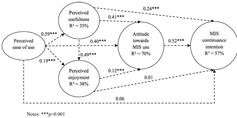
Figure 2: Full group model
